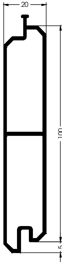
Ref. TPT10 LAMA BISELADA 100x20
